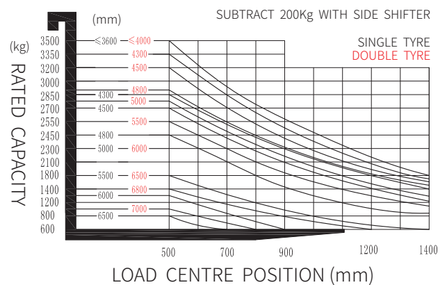
ICE351 RATED CAPACITIES AND LOAD CENTERES GRAPH
