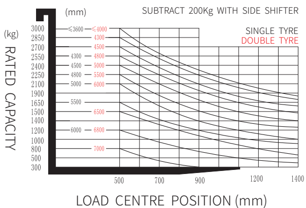
ICE301 RATED CAPACITIES AND LOAD CENTERES GRAPH
